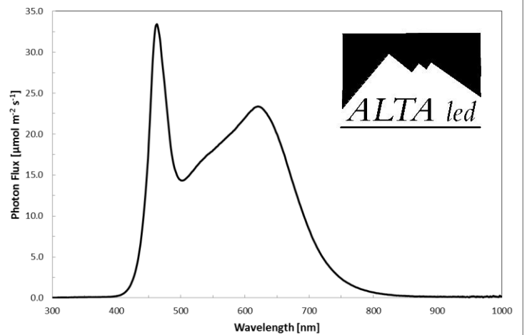
Direct Photon Flux at 3" Distance from HP4S "Veg" Lamp
