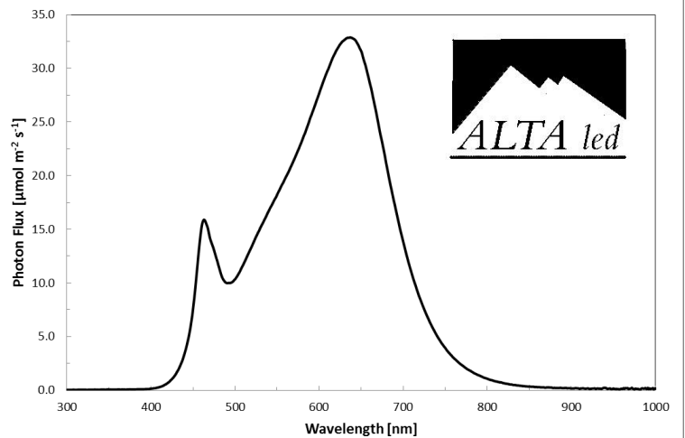
Direct Photon Flux at 3" Distance from HP4S "Grow" Lamp
